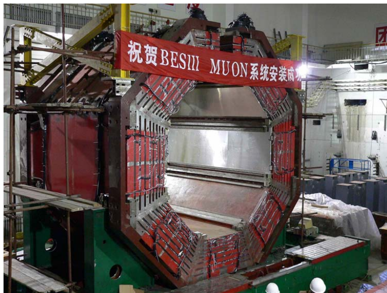
Figure 1. Installed BESIII barrel muon detector.
